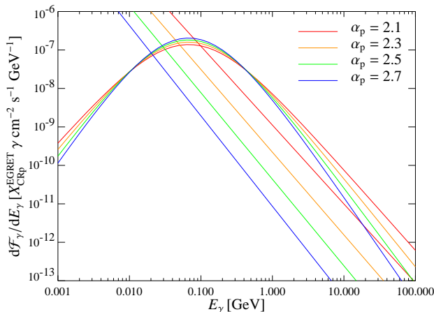
Fig. 1. — Theoretical \gamma -ray spectra of the Perseus cluster resulting from CRp hadronic interactions with the cooling core gas. The assumed CRp spectra are normalized to be marginally consistent with the EGRET E_\gamma > 100 MeV non-detection limits. Results for different proton spectral indices are shown. The \pi^0 -decay bump is clearly visible. Secondary CRes scatter cosmic microwave background photons into the \gamma -ray regime by the inverse Compton process. The resulting power-law emission dominates the low energy part of the spectrum. The CRe population was calculated neglecting synchrotron radiation energy losses. Thus, realistic inverse Compton spectra due to this process will exhibit a lower normalization than displayed here.
