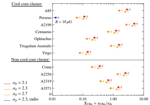
Fig. 2. — EGRET \gamma -ray constraints on the (central) CRp energy density ( \varepsilon_{\text{CRp}} , for various CRp spectral indices) in terms of the cluster central thermal energy density ( \varepsilon_{\text{th}} ) for cooling core and non-cooling core clusters. The constraint from the Perseus cluster radio mini-halo observation is also displayed while assuming a typical cooling core cluster magnetic field strength (blue arrow). If radio mini-halos are entirely produced hadronically by CRps then the constraint derived for the Perseus cluster is an actual measurement for X_{\text{CRp}} and not only an upper limit.
