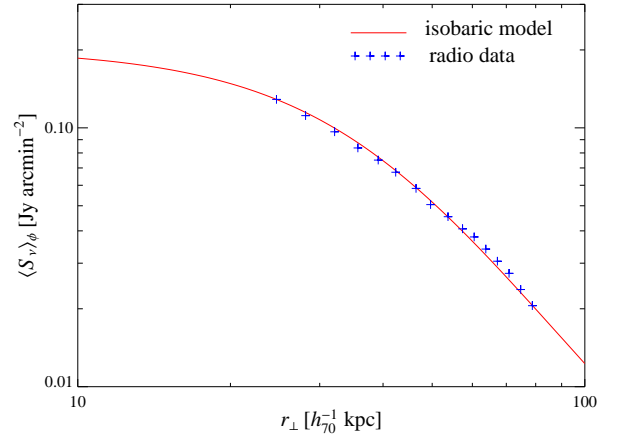
Fig. 5. — Radio emissivity profile of the Perseus mini-halo at 1.4 GHz observed by Pedlar et al. (1990) (crosses) and predicted due to hadronic interactions of CRp by Pfrommer & Enßlin (2004a). Both the required CRp scaling ratio X_{\text{CRp}} \simeq 2\% and the morphological match of the observed and predicted radio emissivities strongly indicate the hadronic origin of radio mini-halos.
