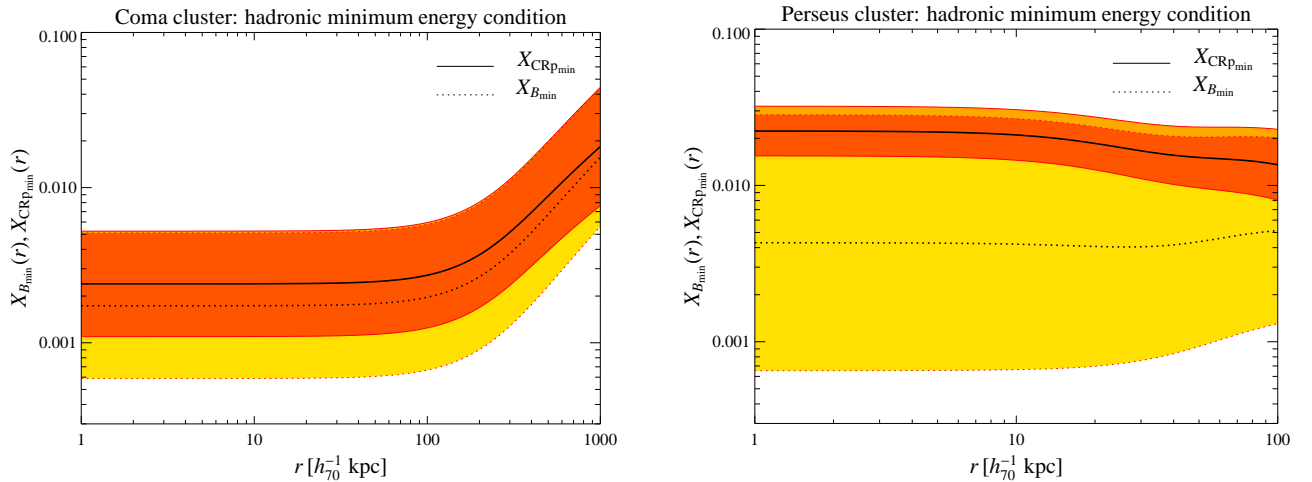
Fig. 6. — Profiles of the CRp-to-thermal energy density X_{\text{CRp}_{\min}}(r) (solid) and magnetic-to-thermal energy density X_{B_{\min}}(r) (dotted) as a function of deprojected radius are shown. The different energy densities are obtained by means of the hadronic minimum energy criterion. The left panel shows profiles of the Coma cluster while the right panel represents profiles of the Perseus cluster. The light shaded areas represent the logarithmic tolerance regions of X_{B_{\min}}(r) and X_{\text{CRp}_{\min}}(r) , respectively, while the dark shaded regions indicate the overlap and thus the possible equipartition regions in the quasi-optimal case.
